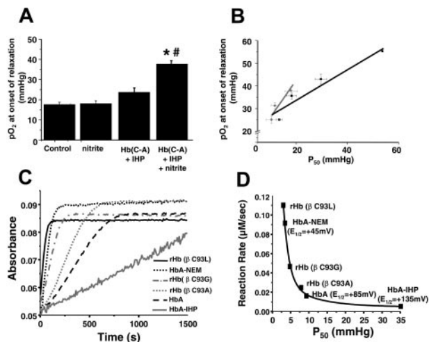
Figure 4. \beta 93cys residue controls nitrite reductase activity of Hb. (A) Hb(C \rightarrow A) potentiates nitrite-dependent relaxation. Final concentrations: nitrite (2 \mu M), Hb(C \rightarrow A) (25 \mu M), and IHP (625 \mu M). * P < .001 relative to nitrite alone. # P < .01 relative to Hb(C \rightarrow A) + IHP. Data represent mean \pm SEM ( n = 3–5). (B) Relationship between P_{50} of HbA (■) or Hb(C \rightarrow A) (●) and the oxygen tension at the initiation of vessel dilation in the presence of nitrite (2 \mu M). Data for HbA are taken from Figure 3C. P_{50} was modulated by the addition of varying amounts of IHP and was determined under identical buffer, pH, temperature, and P_{CO_2} conditions as for vessel dilation studies. A linear relationship between P_{50} and oxygen tension at the onset of relaxation was observed for both Hbs (black line: y = 20.7 + 0.67x ; r = 0.96 ; gray line: y = 11.6 + 1.48x ; r = 0.94 ). Data represent mean \pm SEM ( n = 3–6). (C) Representative reaction traces for metHb formation from the reaction between nitrite and various deoxyHbs (experiments performed under anoxic conditions). (D) Relationship between Hb P_{50} and rate of nitrite reduction. Shown are the best fit line ( R^2 = 0.99 ) and the average redox potentials ( E_{1/2} ) from values in the literature. 37,40,42
